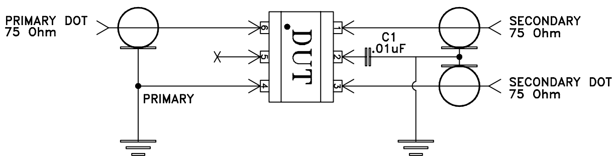
Schematic Diagram
