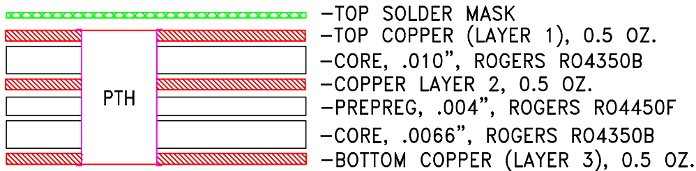
Structural Diagram
