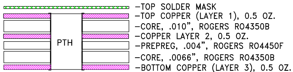
Stack-Up Diagram
