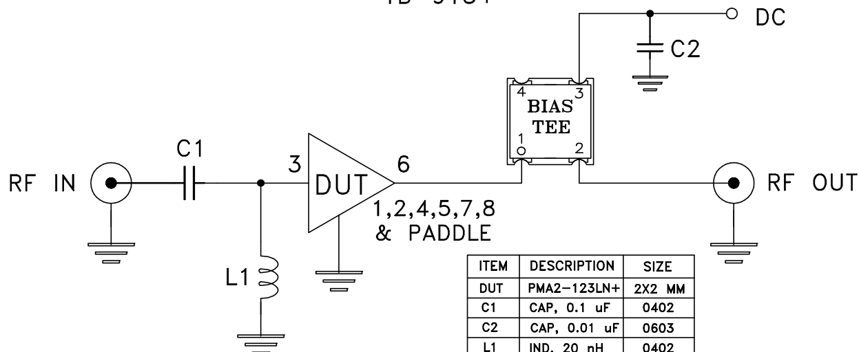
Schematic Diagram
