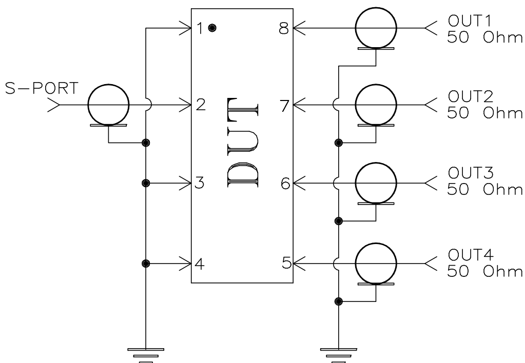
Schematic Diagram
