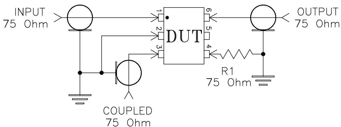
Schematic Diagram
