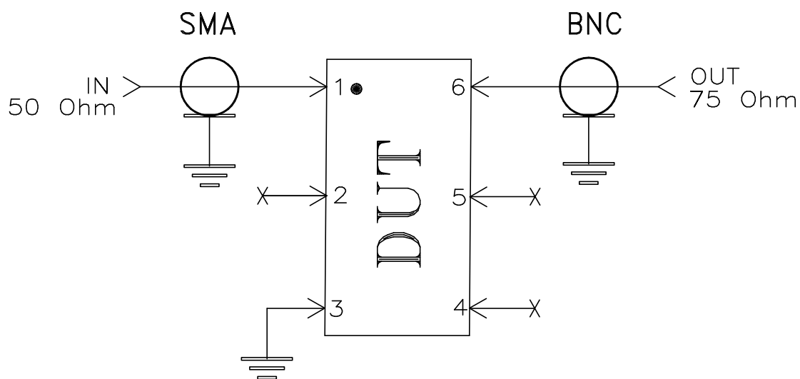
Schematic Diagram
