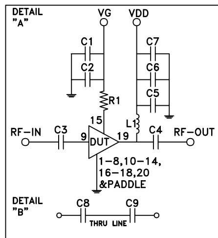
SCHEMATIC DIAGRAM
