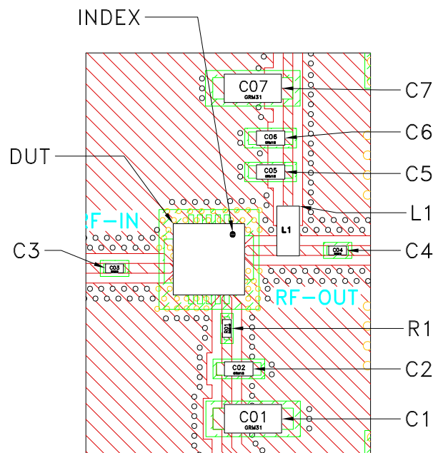
DETAIL "A" LOCATION OF UNITS COMPONENTS (SCALE 3:1)
