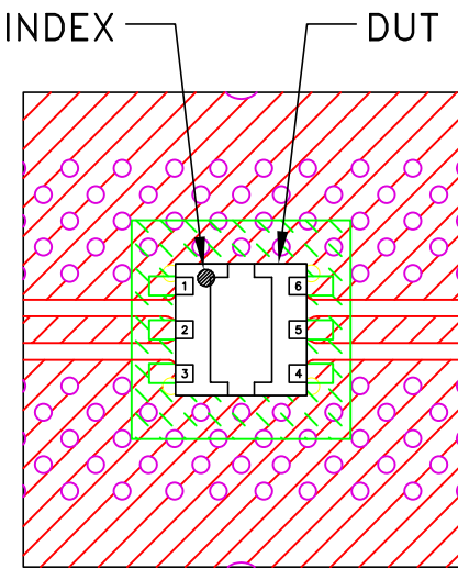
DETAIL "A" (SCALE 5:1)
