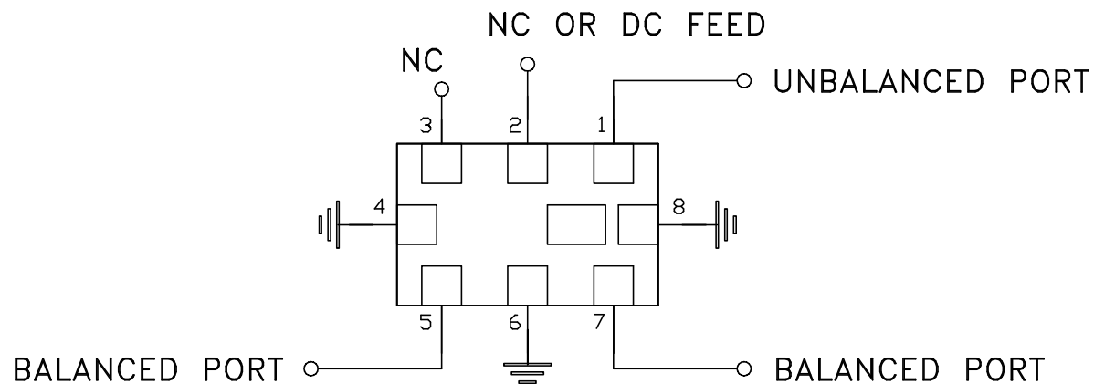
Schematic Diagram
