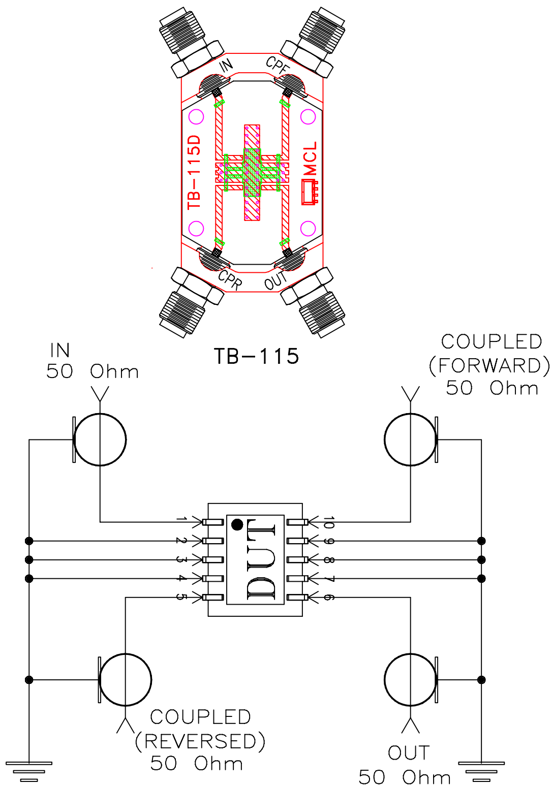
Schematic Diagram
