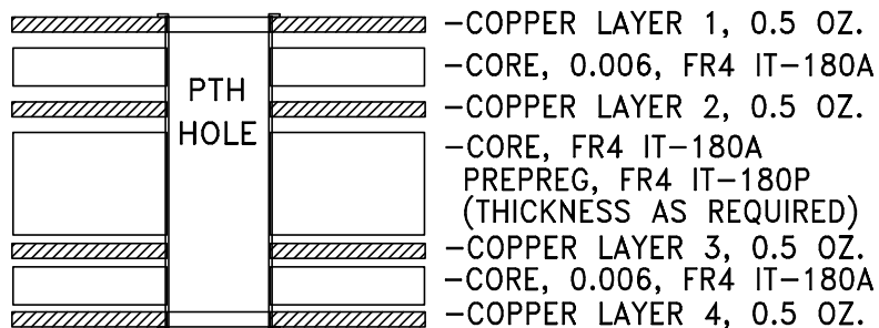
Stack-up Diagram
