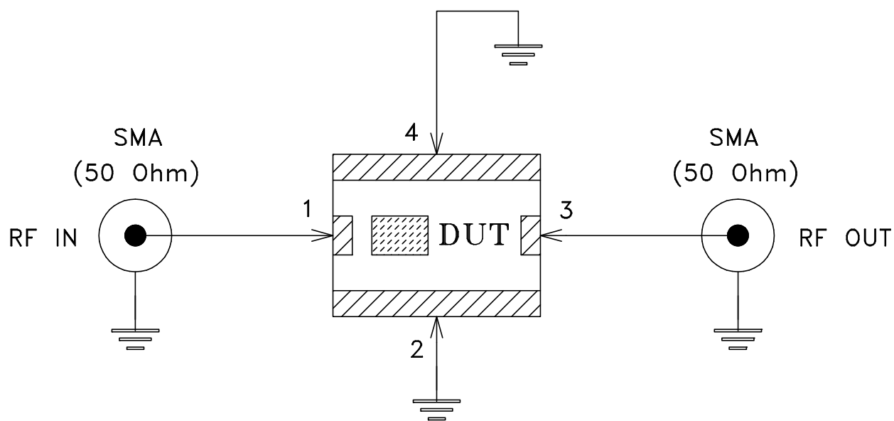
Schematic Diagram
