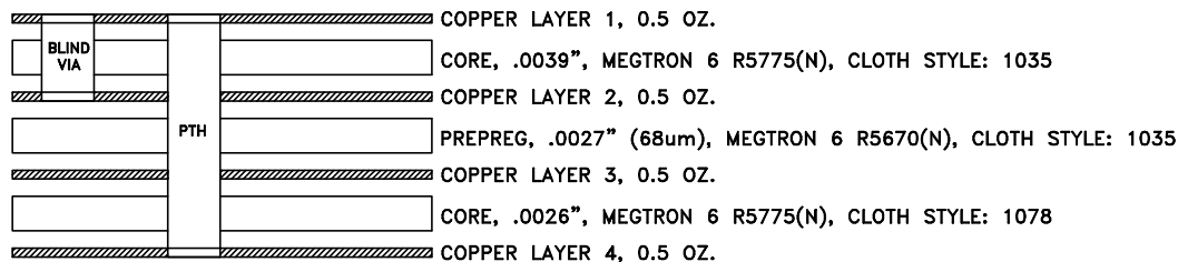
STACK-UP DIAGRAM
