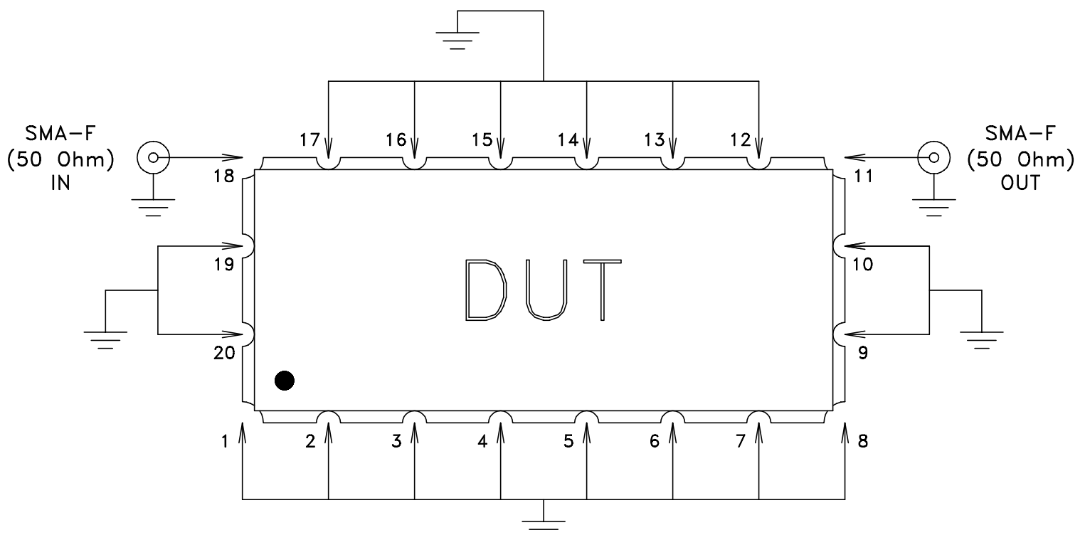
Schematic Diagram
