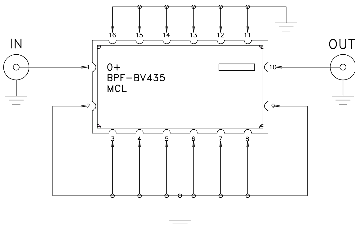
Schematic Diagram
