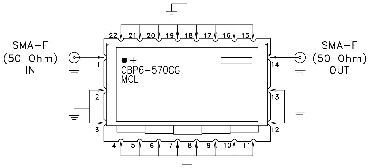
Schematic diagram
