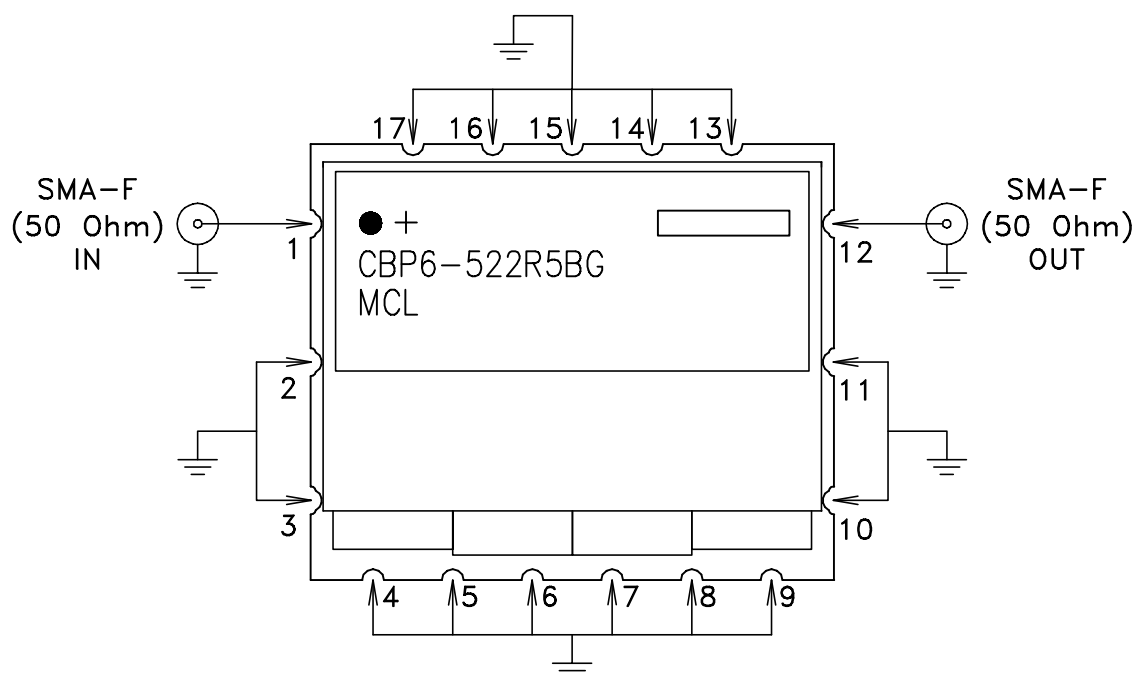
Schematic diagram
