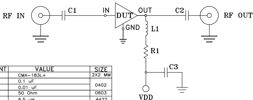
Schematic Diagram
