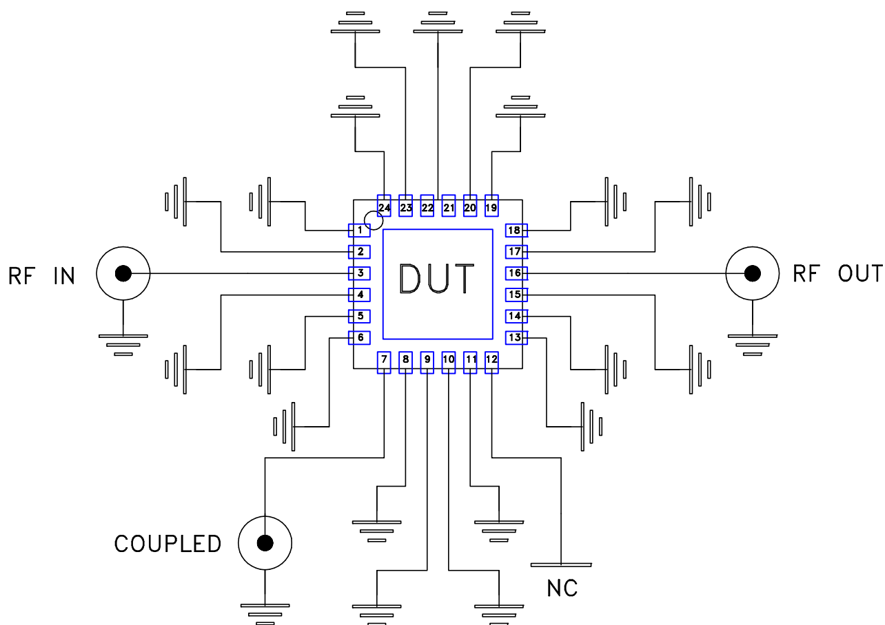
Schematic Diagram
