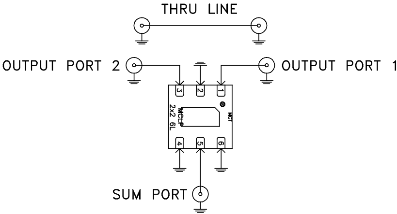
SCHEMATIC DIAGRAM (SCALE 5:1)
