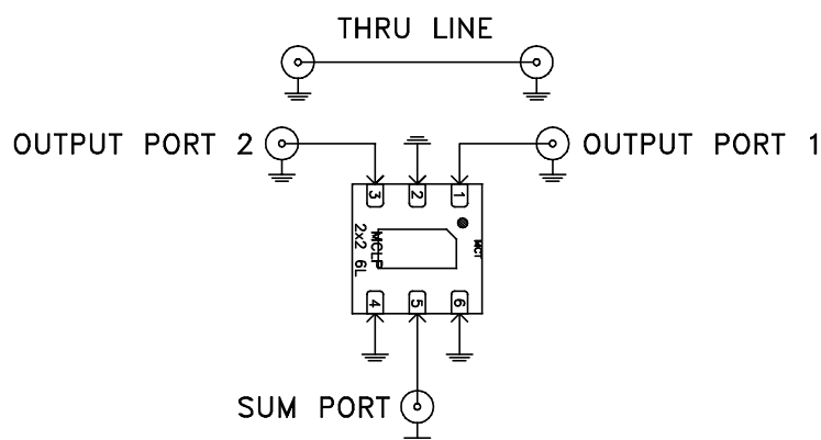
SCHEMATIC DIAGRAM (SCALE 5:1)
