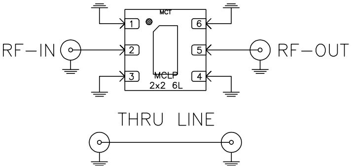
SCHEMATIC DIAGRAM
