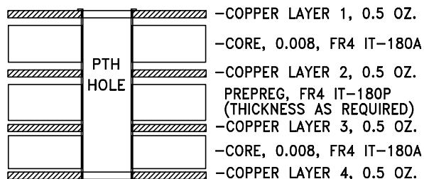
Stack-up Diagram
