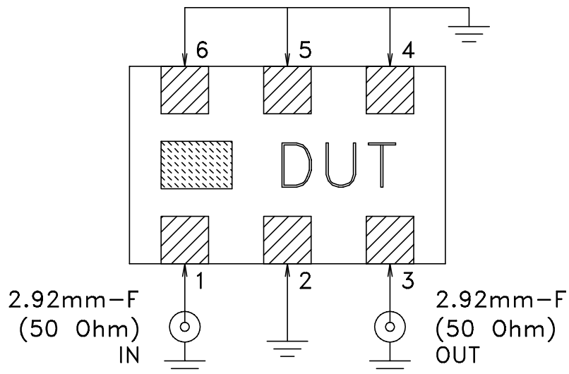
Schematic diagram
