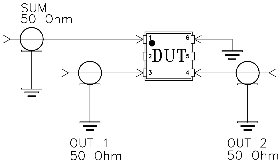
Schematic Diagram
