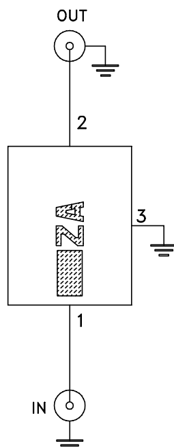
Schematic Diagram
