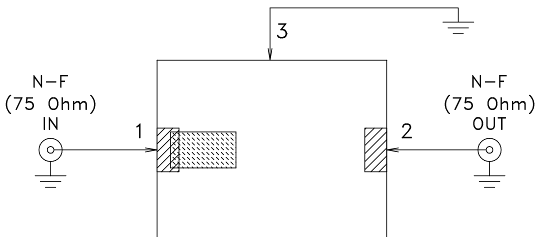
Schematic Diagram
