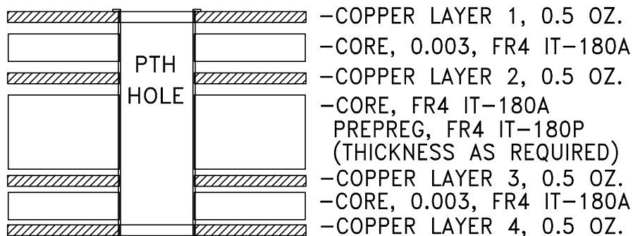
Stack-up Diagram
