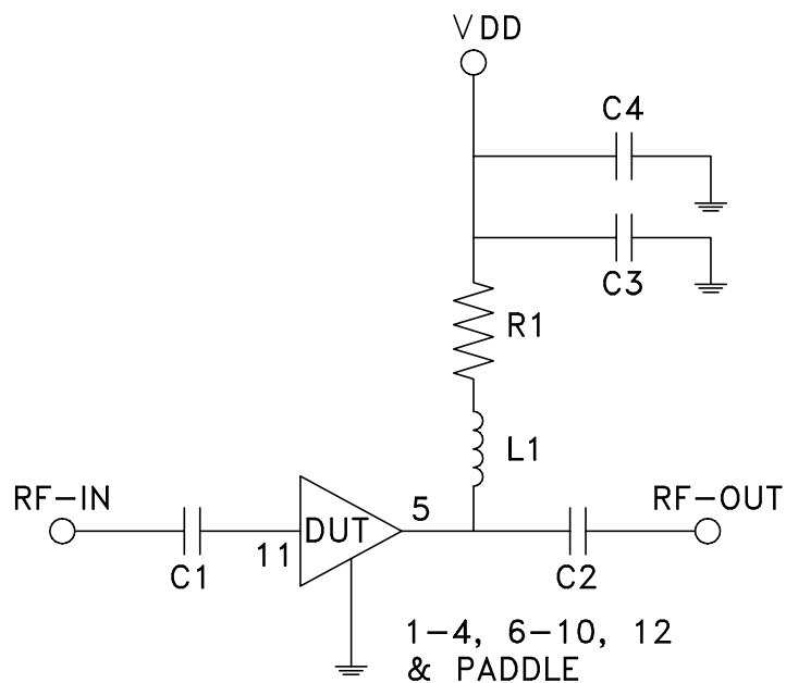
SCHEMATIC DIAGRAM
