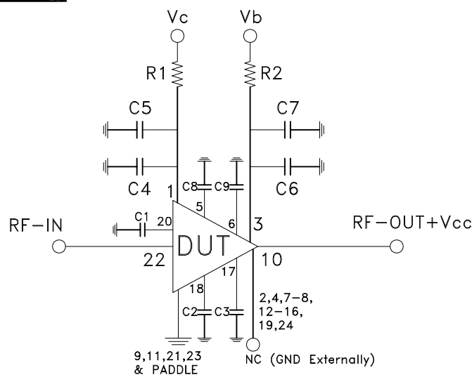
SCHEMATIC DIAGRAM
