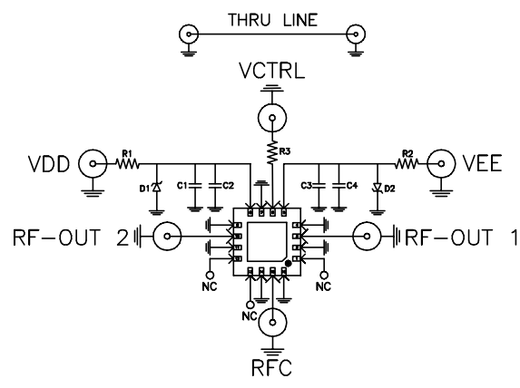
SCHEMATIC DIAGRAM (SCALE 3:1)
