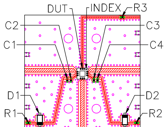
DETAIL "A" LOCATION OF COMPONENTS ON THE PCB (SCALE 1.5:1)
