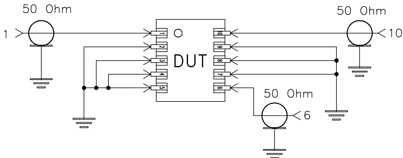
Schematic Diagram
