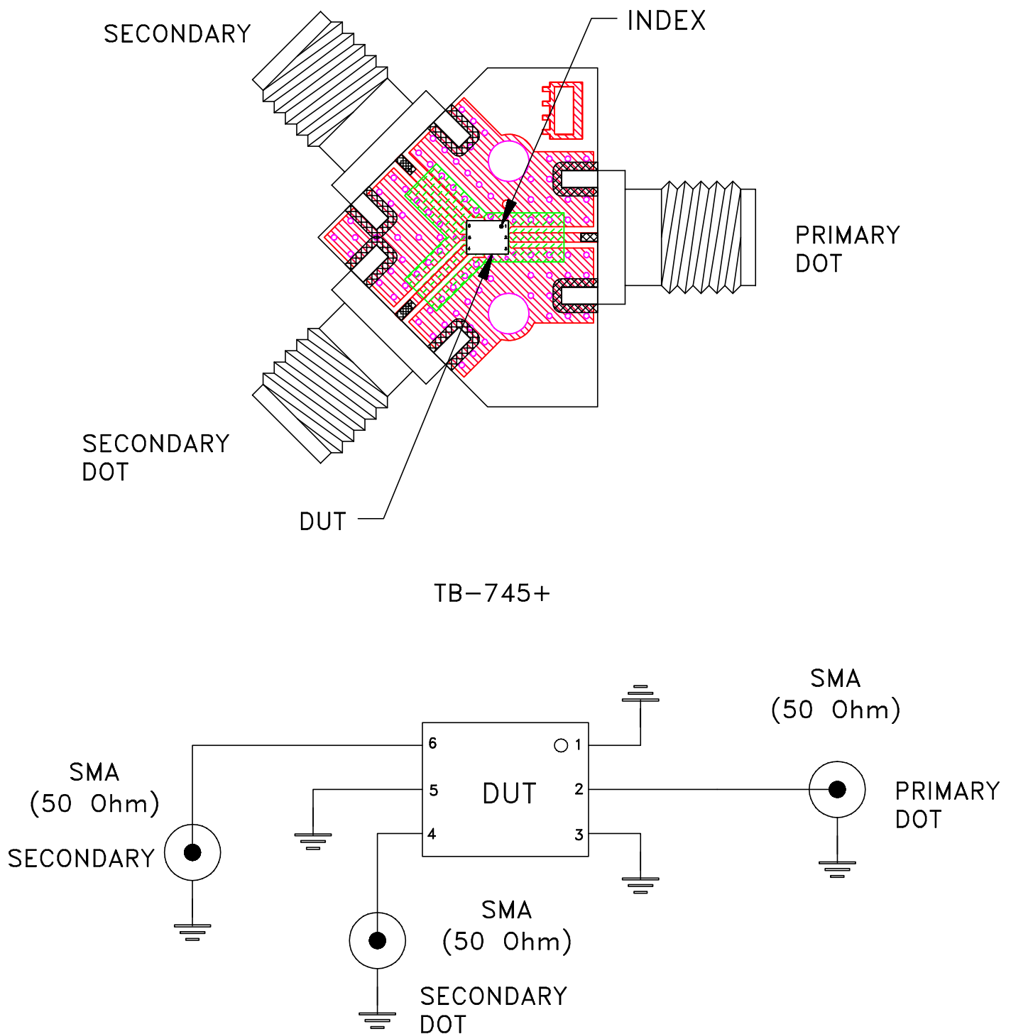
Schematic Diagram
