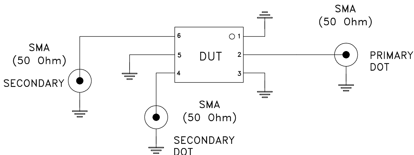
Schematic Diagram
