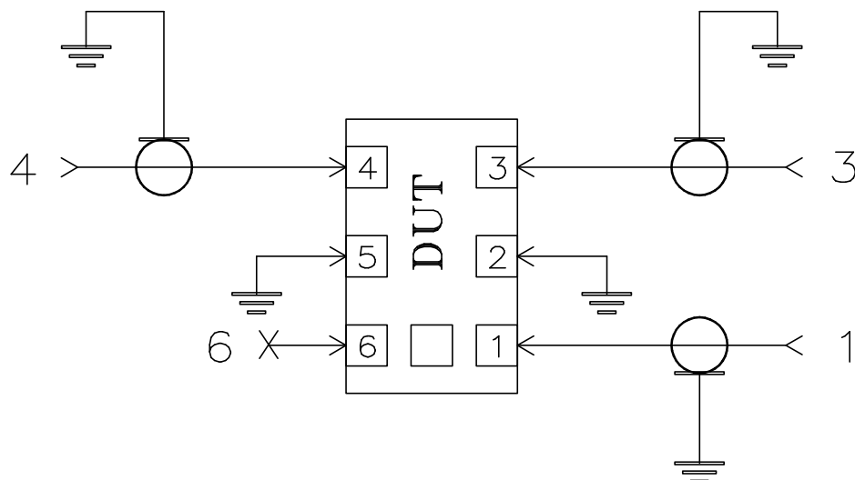
Schematic Diagram
