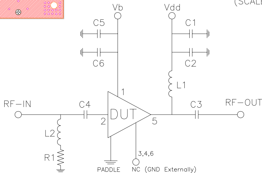
SCHEMATIC DIAGRAM
