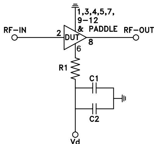
SCHEMATIC DIAGRAM
