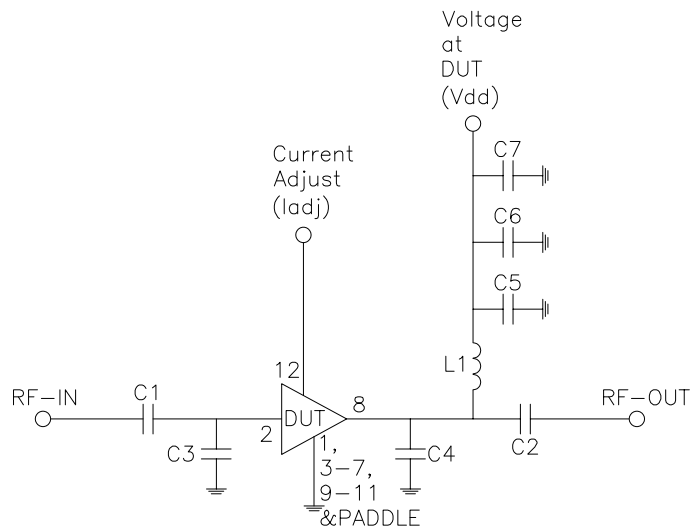
SCHEMATIC DIAGRAM
