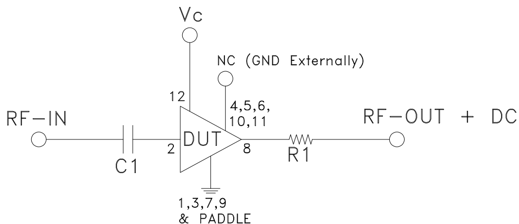
SCHEMATIC DIAGRAM
