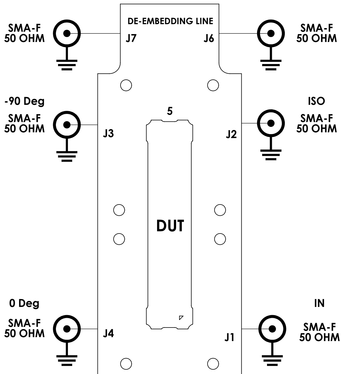
TB-QCH-63B+ Schematic Diagram
