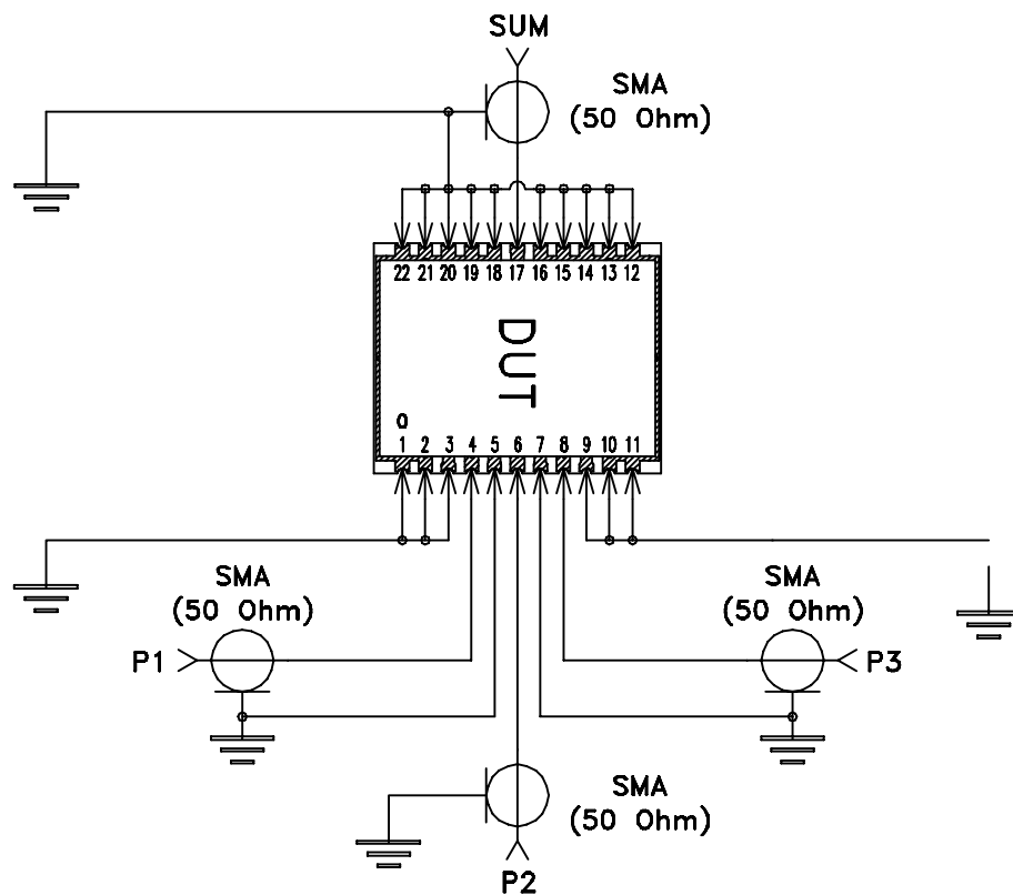
Schematic Diagram
