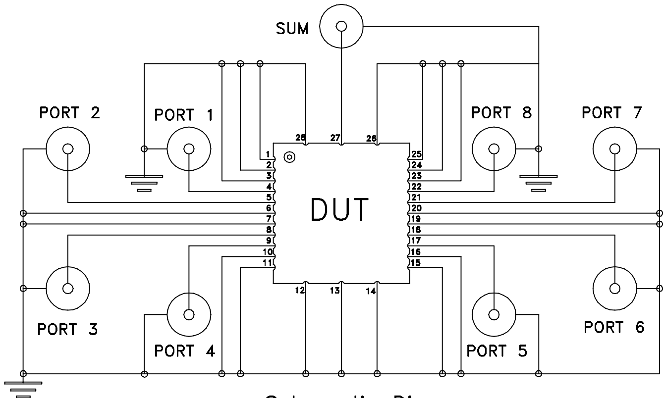
Schematic Diagram
