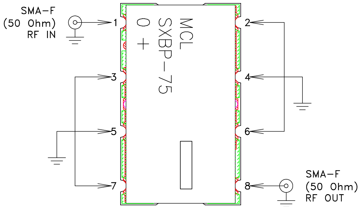
Schematic diagram
