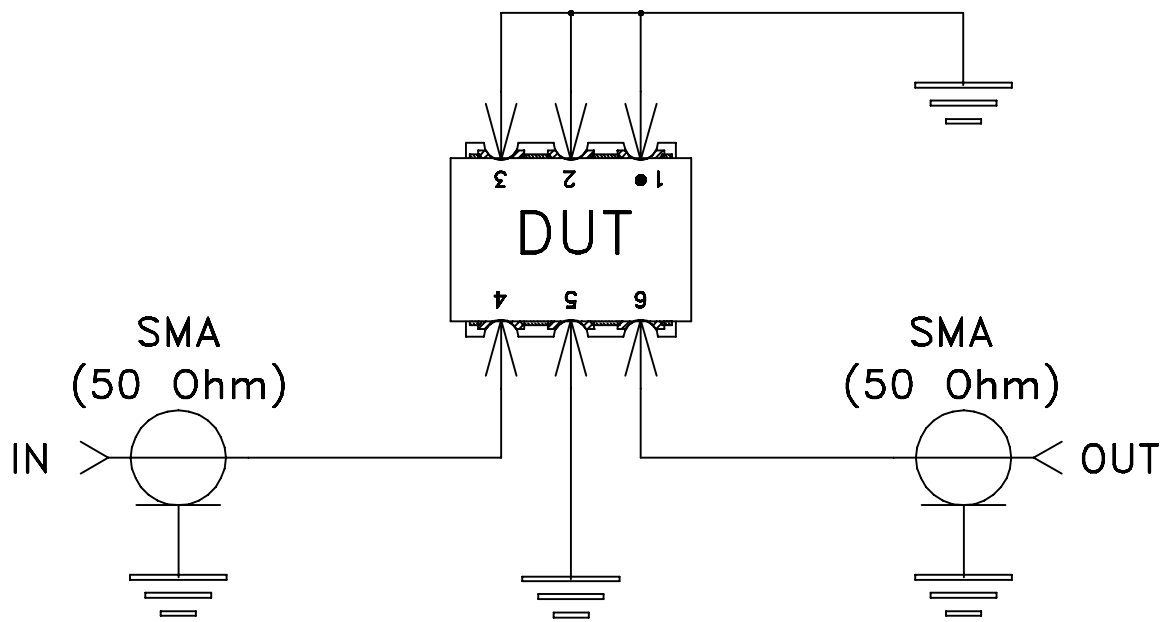
Schematic Diagram
