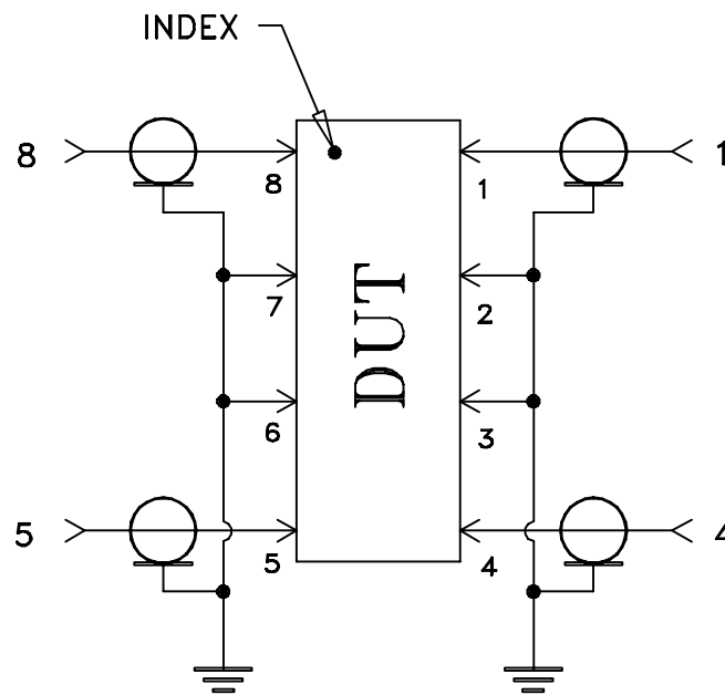
Schematic Diagram
