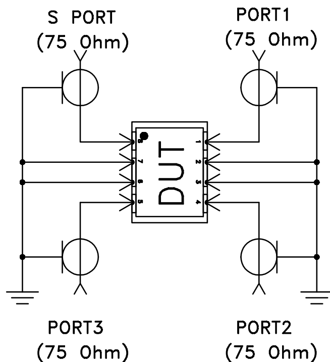
Schematic Diagram
