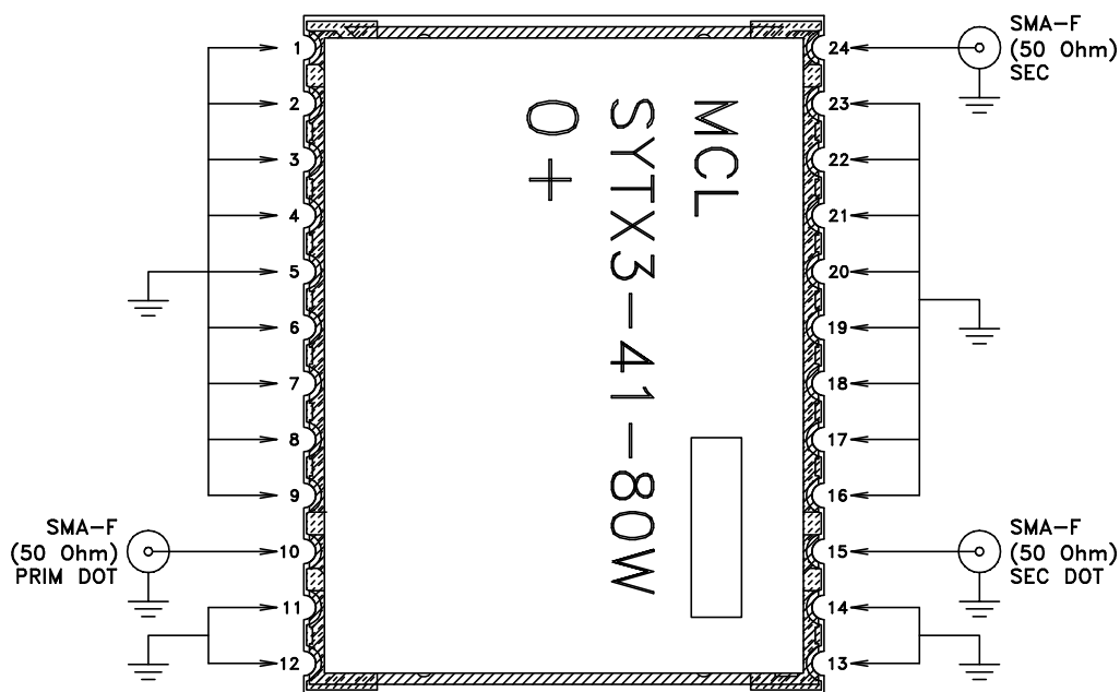
Schematic diagram
