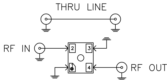
SCHEMATIC DIAGRAM (SCALE 5:1)
